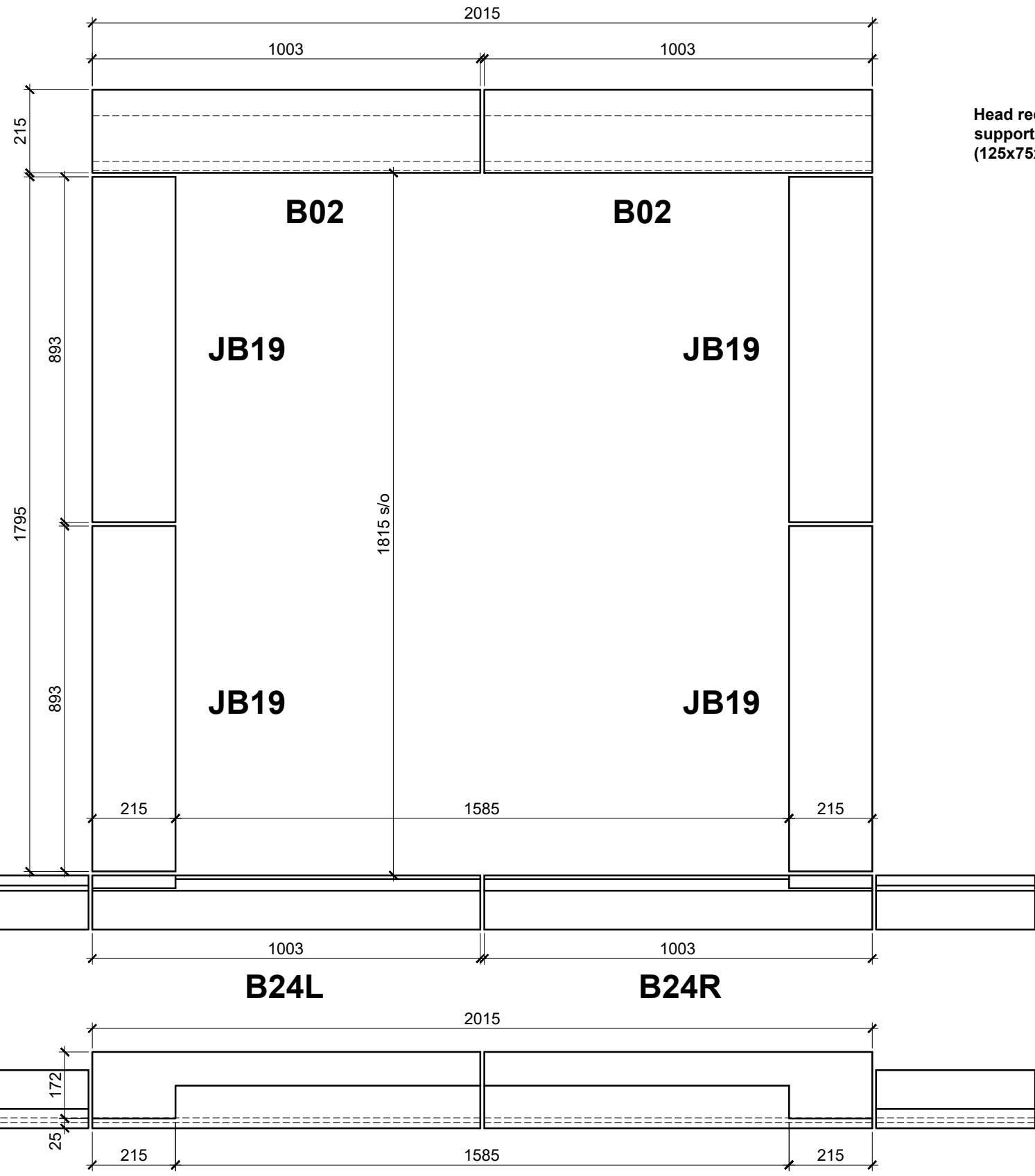
Plan View Unit Ref: B24LT25068A (46kg) Plan View Unit Ref: B24RT25068B (46kg)
